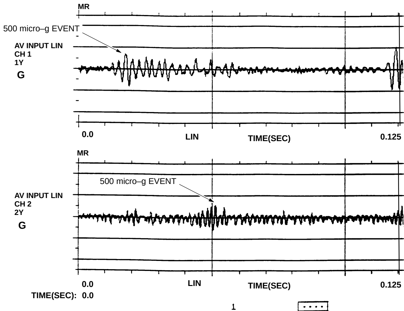
ACCELERATION TIME HISTORY ILLUSTRATION A-3
